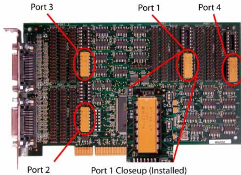
Figure 3 Termination Sockets
