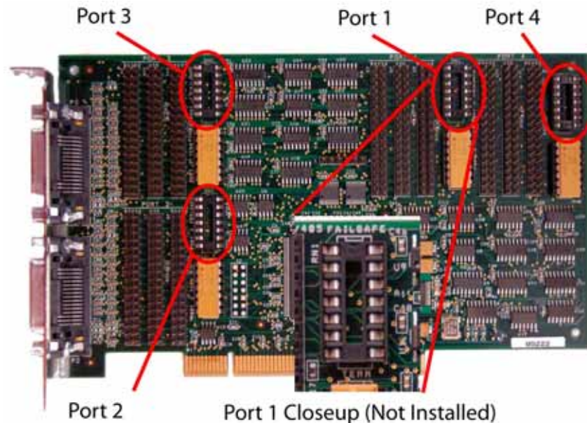
Figure 4 Fail Safe Biasing Sockets
