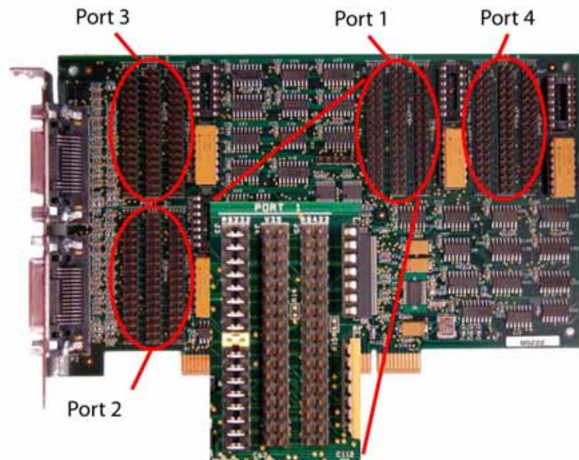
Port 1 Closeup (RS-232 Selected)
